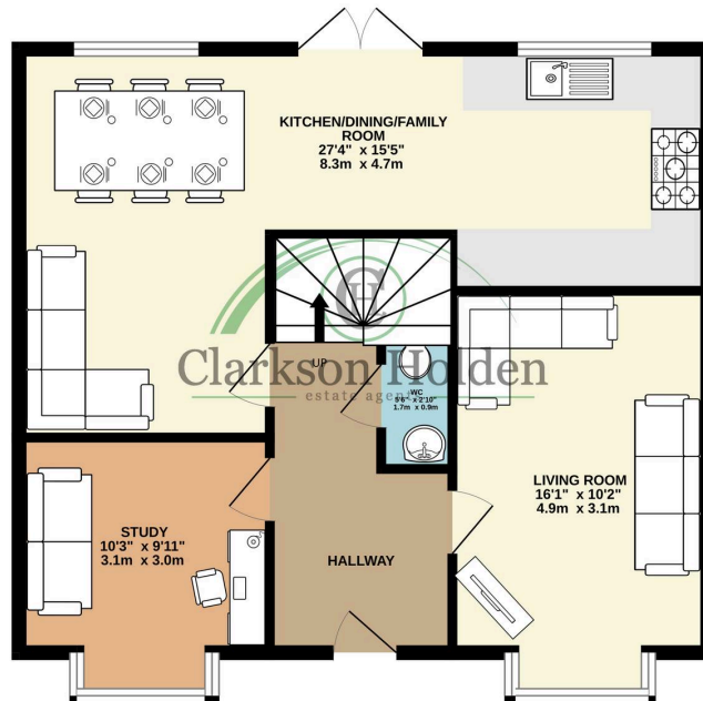
GROUND FLOOR 673 sq.ft. (62.5 sq.m.) approx.
